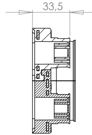
SECTION C-C
