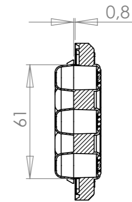
SECTION B-B
